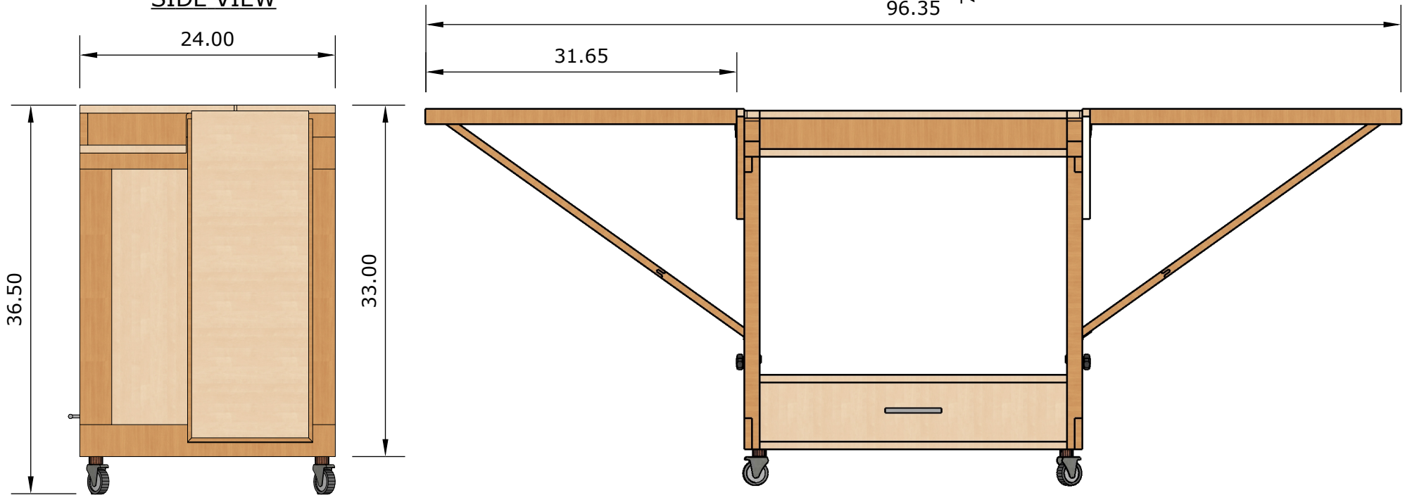
SIDE VIEW
